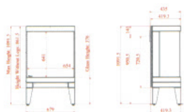
Back Chimney Configuration
