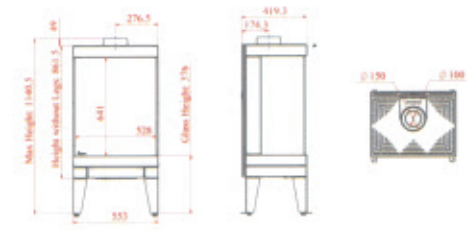
Top Chimney Configuration
