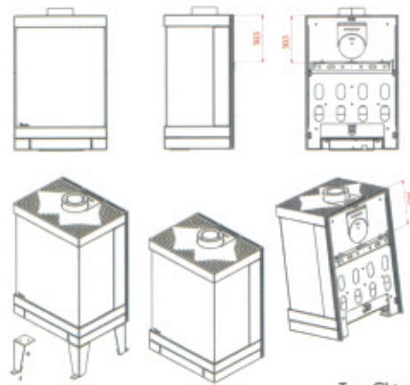
Top Chimney Configuration
