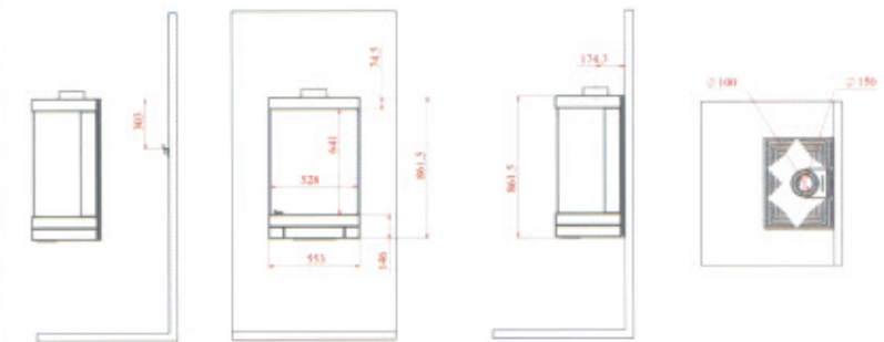
Top Chimney Configuration
