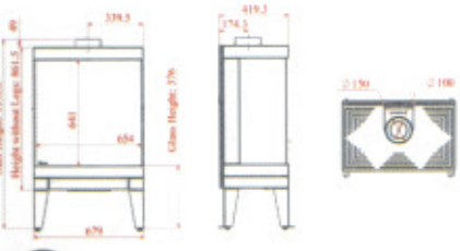
Top Chimney Configuration
